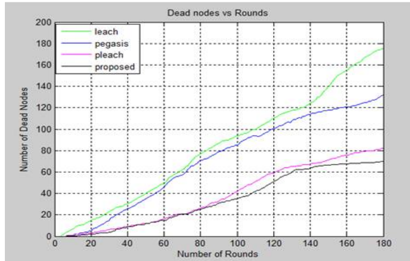
Figure 1 -Number of dead nodes vs Rounds
