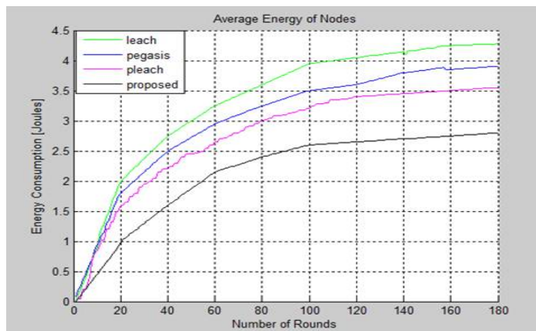
Figure2- Energy consumption vs Rounds
