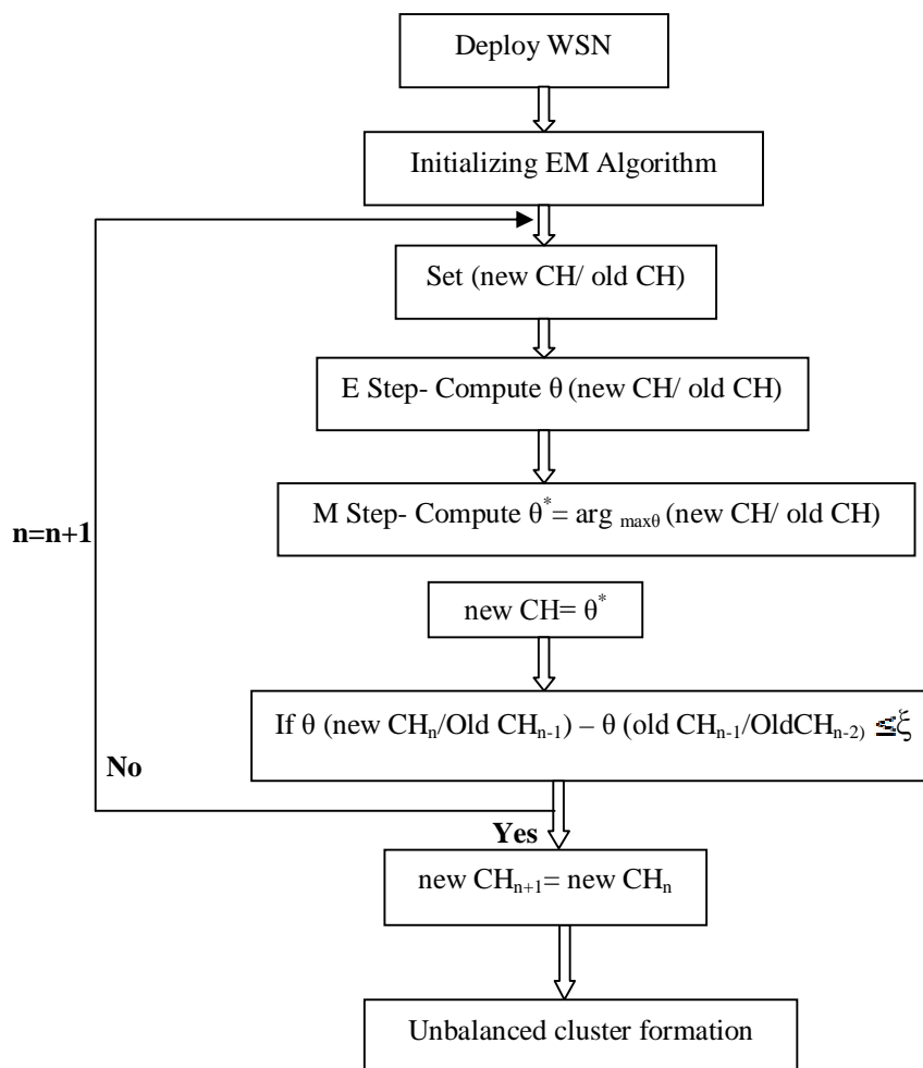
Figure 1. Flow diagram of algorithm
